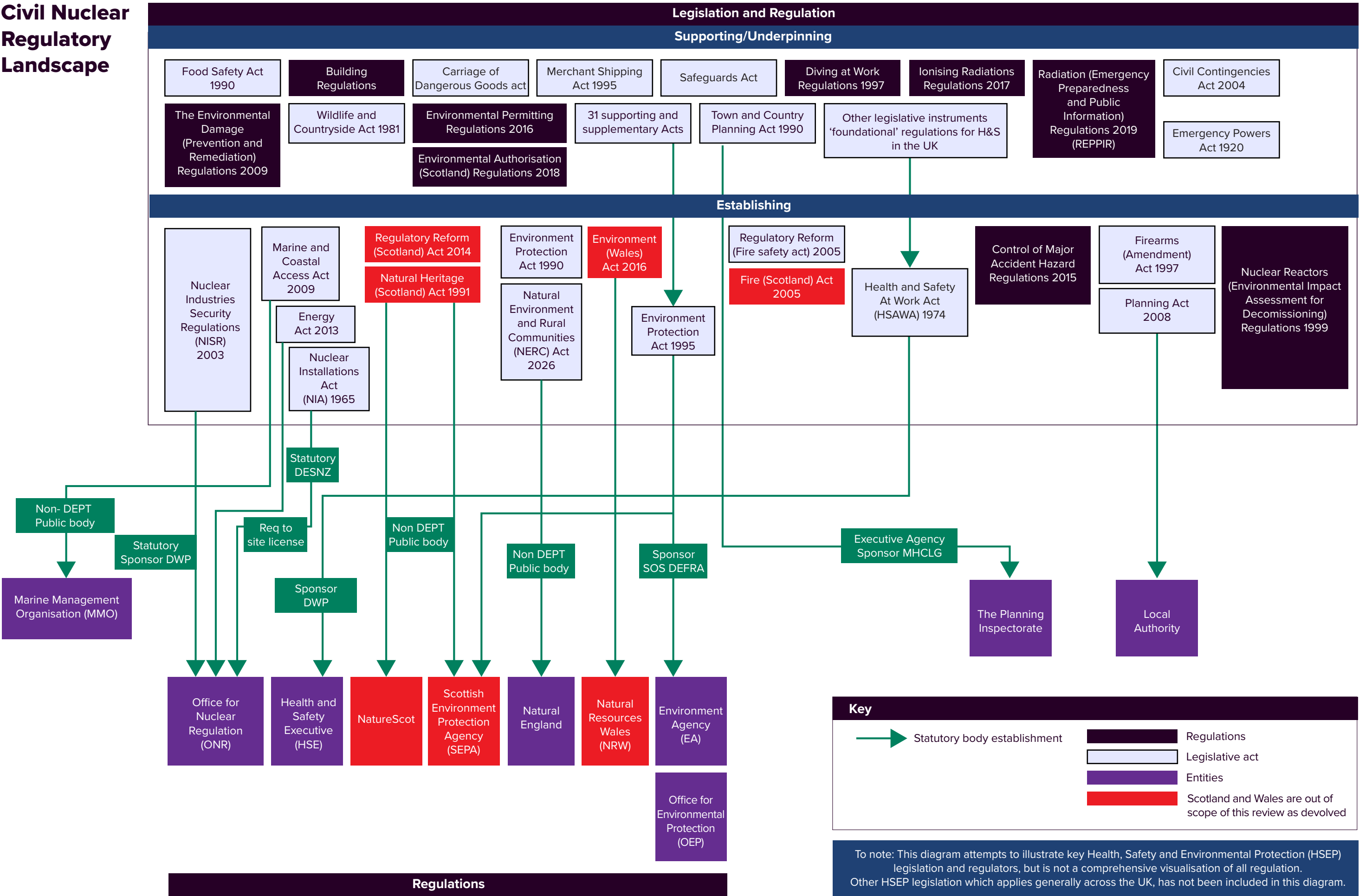
Figure 3 – The civil nuclear regulatory landscape
