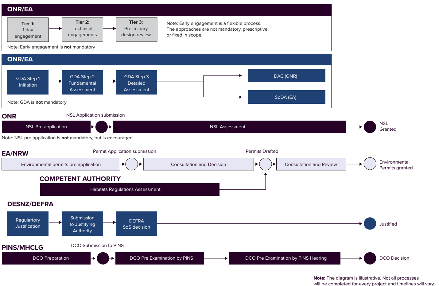
Figure 5 - UK Regulatory Processes for New Nuclear Build
